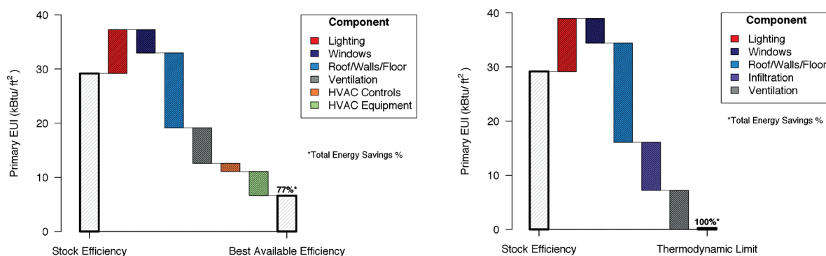
Figure 5.9 Use of the most efficient wall, window, and HVAC equipment now available could reduce commercial heating 77%. Increased lighting efficiency increases the load met by heating systems.
