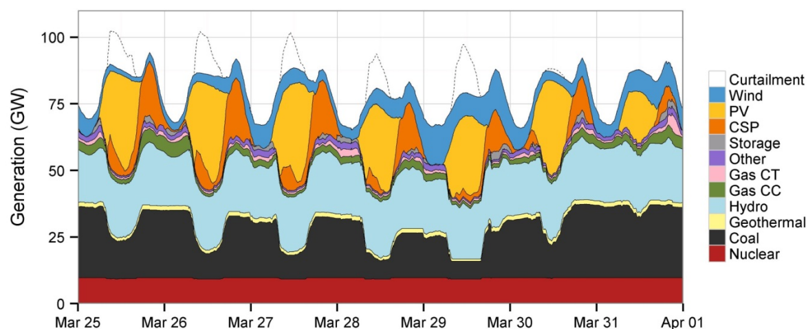
Figure 3. Simulated impacts of obtaining 33% energy from wind and solar
