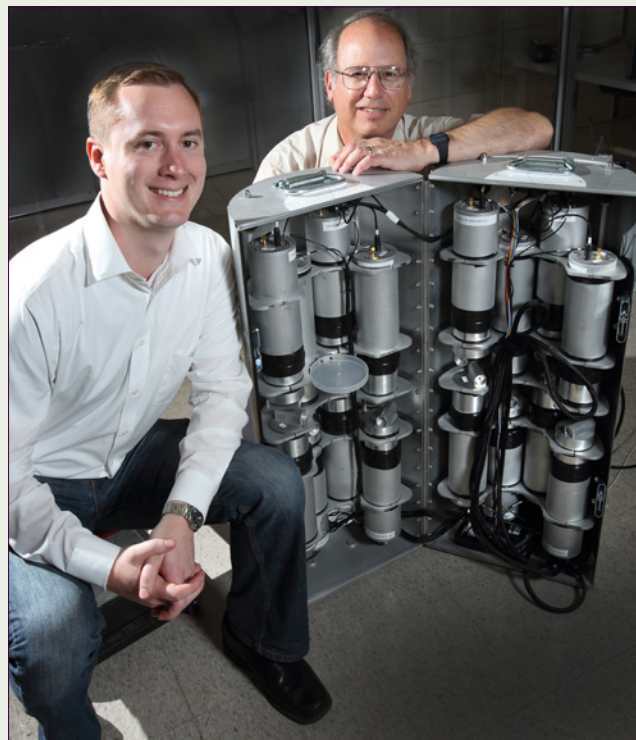
SNL physicists Mark Gerling (left) and John Goldsmith with the MINER detection system opened to show the 16 liquid scintillator detector cells. Photo by Dino Vournas
