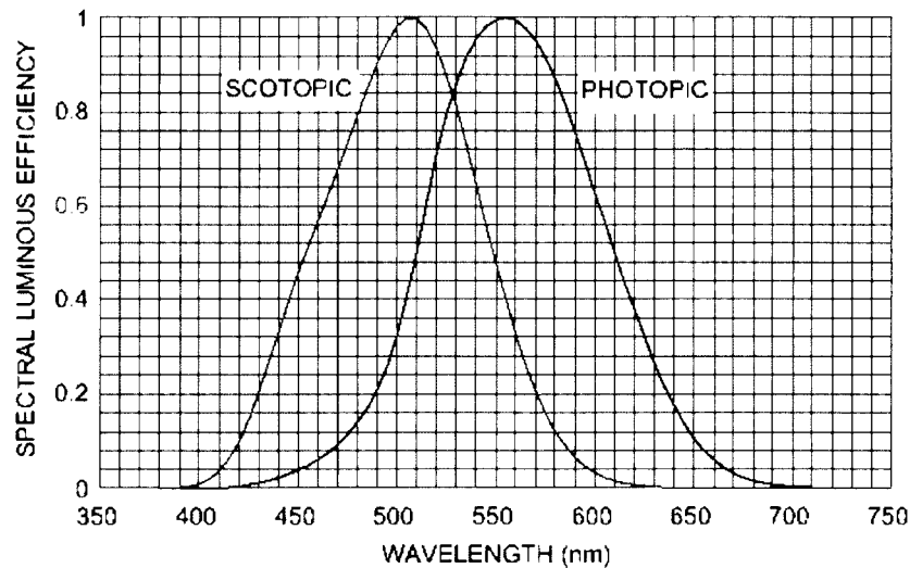
Figure 4-1: Photopic and Scotopic V- \lambda Curves
