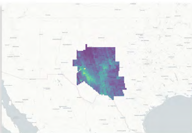
Aggregate of emissions in Permian for 2022
