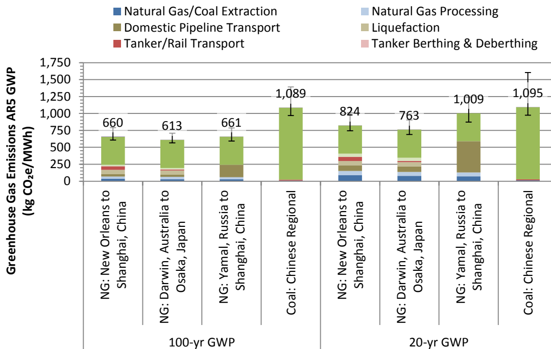
Figure 4: Life Cycle GHG Emissions for Natural Gas and Coal Power in Asia 297
