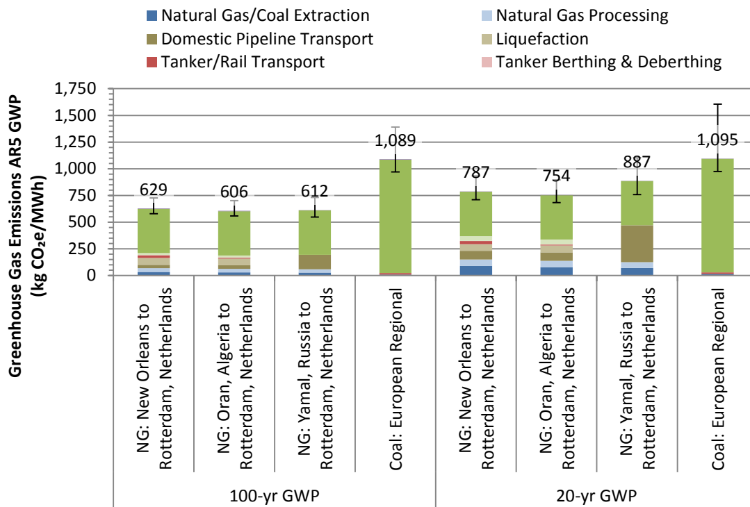
Figure 3: Life Cycle GHG Emissions for Natural Gas and Coal Power in Europe 296
