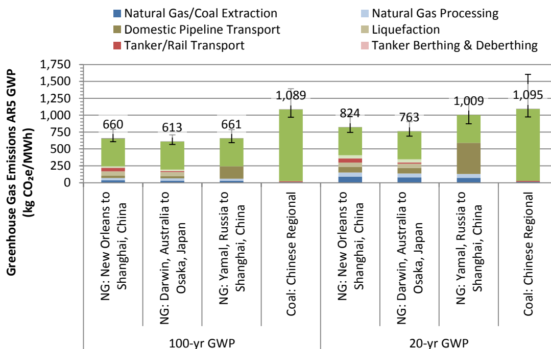
Figure 2: Life Cycle GHG Emissions for Natural Gas and Coal Power in Asia 245
