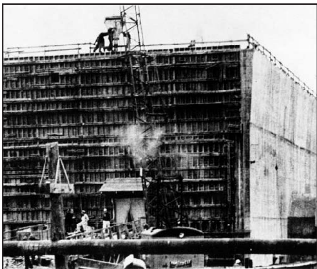
Chemical Separation Plant (Queen Mary) Under Construction at Hanford. Reprinted from Richard G. Hewlett and Oscar E. Anderson, Jr., The New World, 1939-1946 , Volume I of A History of the United States Atomic Energy Commission (University Park: Pennsylvania State University Press, 1962).
