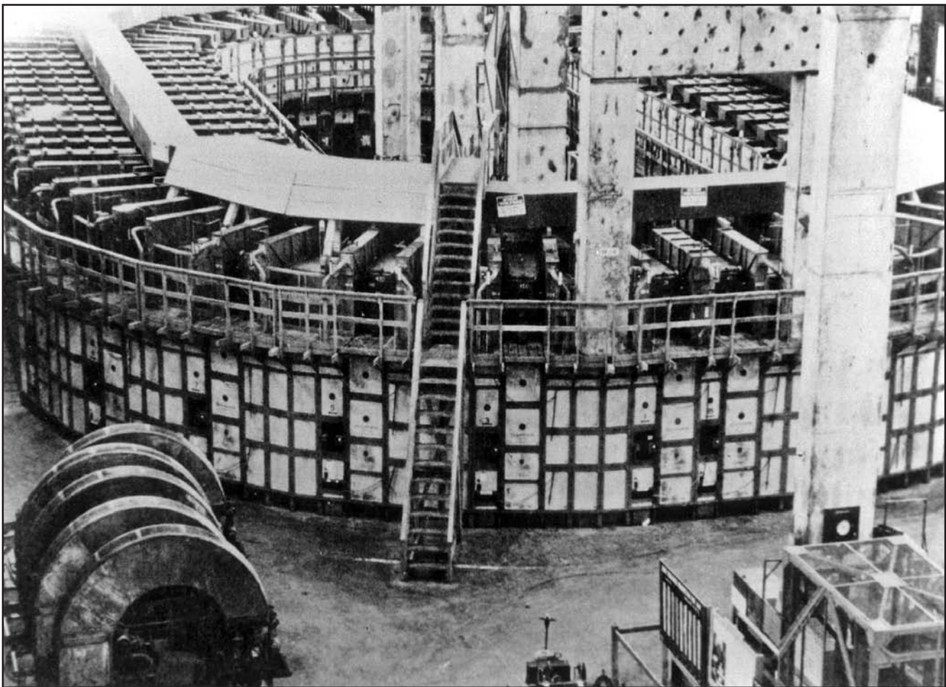
Y-12 Alpha Racetrack at Clinton. Spare vacuum tanks in Left Foreground. Reprinted from Richard G. Hewlett and Oscar E. Anderson, Jr., The New World, 1939-1946 , Volume I of A History of the United States Atomic Energy Commission (University Park: Pennsylvania State University Press, 1962).
