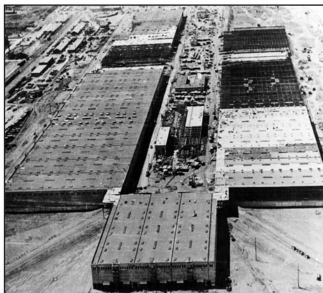
K-25 from Opposite End. White Building in Center of Previous Picture Discernible at Far End. Reprinted from Richard G. Hewlett and Oscar E. Anderson, Jr., The New World, 1939-1946 , Volume I of A History of the United States Atomic Energy Commission (University Park: Pennsylvania State University Press, 1962).
