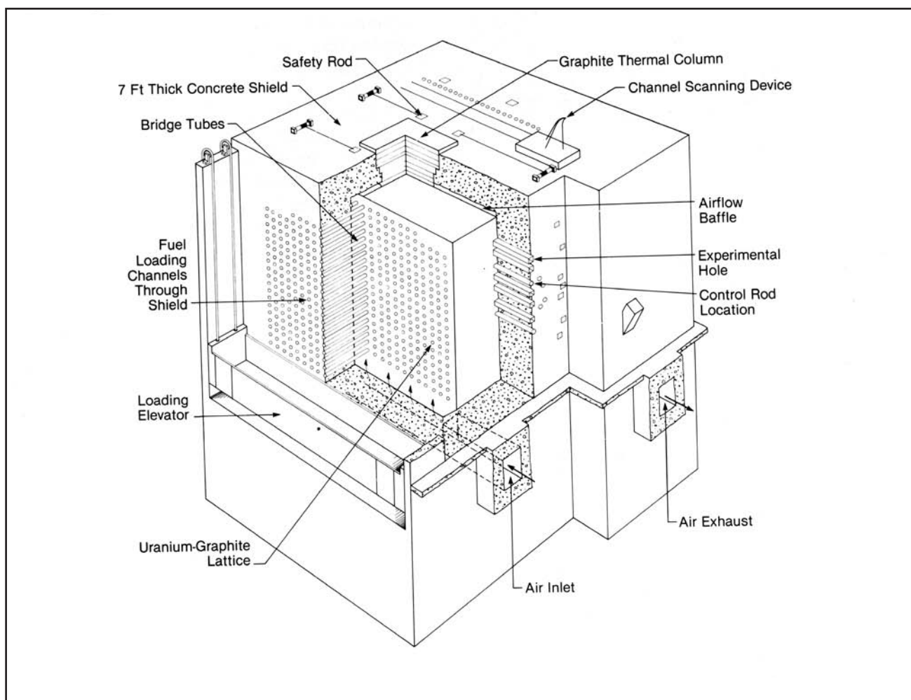
Air-Cooled Pile Built in X-10 Area at Clinton. Reprinted from Richard G. Hewlett and Oscar E. Anderson, Jr., The New World, 1939-1946 , Volume I of A History of the United States Atomic Energy Commission (University Park: Pennsylvania State University Press, 1962).
