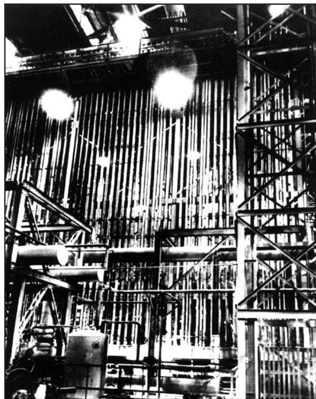
Section of S-50 Liquid Thermal Diffusion Plant at Clinton. Reprinted from Richard G. Hewlett and Oscar E. Anderson, Jr., The New World, 1939-1946 , Volume I of A History of the United States Atomic Energy Commission (University Park: Pennsylvania State University Press, 1962).
