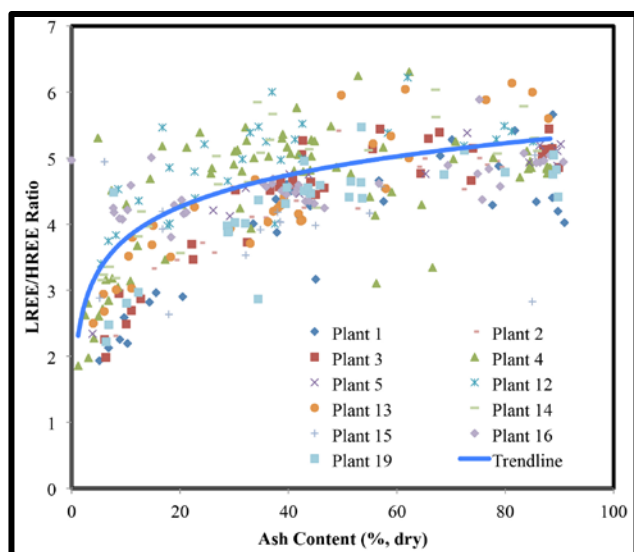
Figure 8. LREE/HREE vs. Coal Ash Content
