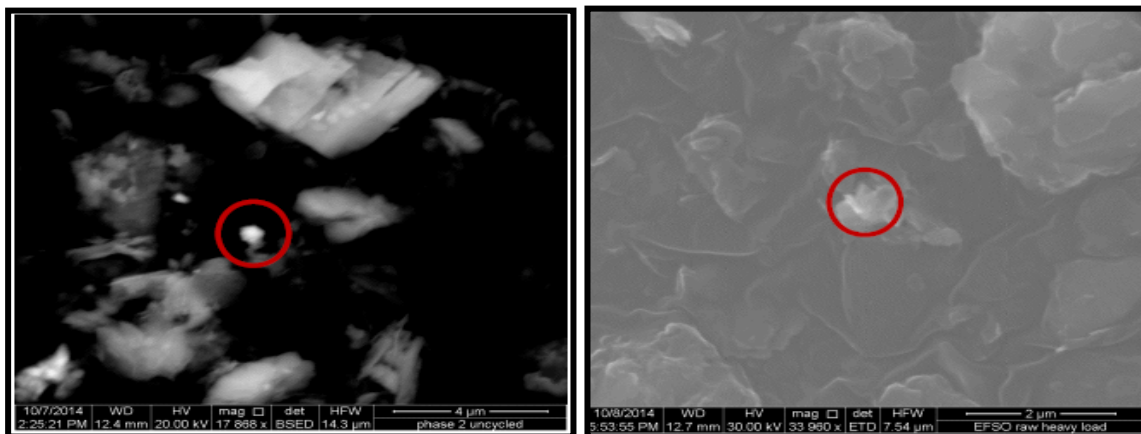
Figures 9 (a) and (b). Scanning electron microscope images of bastnaesite (a) and monazite (b) particles in the reject generated from the processing of Fireclay seam coal.
