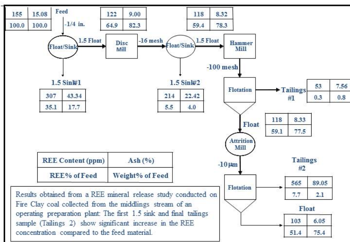
Figure 7. Mineral Release Test, Fire Clay Coal
