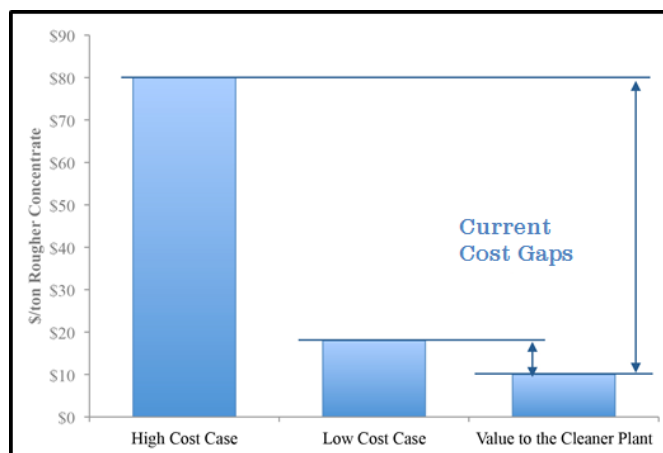
Figure 14. Rougher plant production costs for low-assay REE concentrates from coal compared with a value required as feedstock for the cleaner plant
