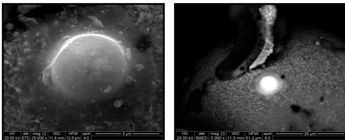
Figures 9 (c) and (d). Cenospheres in fly ash with a monazite particle trapped inside. Secondary and backscatter images of a La, Ce, Nd, Pr, P-rich particle. Chemistry is consistent with monazite. Spherical particle is possibly melted monazite. Note that each image is at a different magnification.
