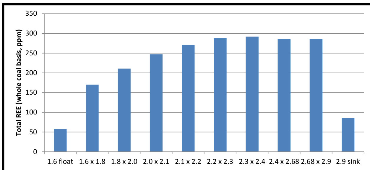
Figure 6. Washability Summary
