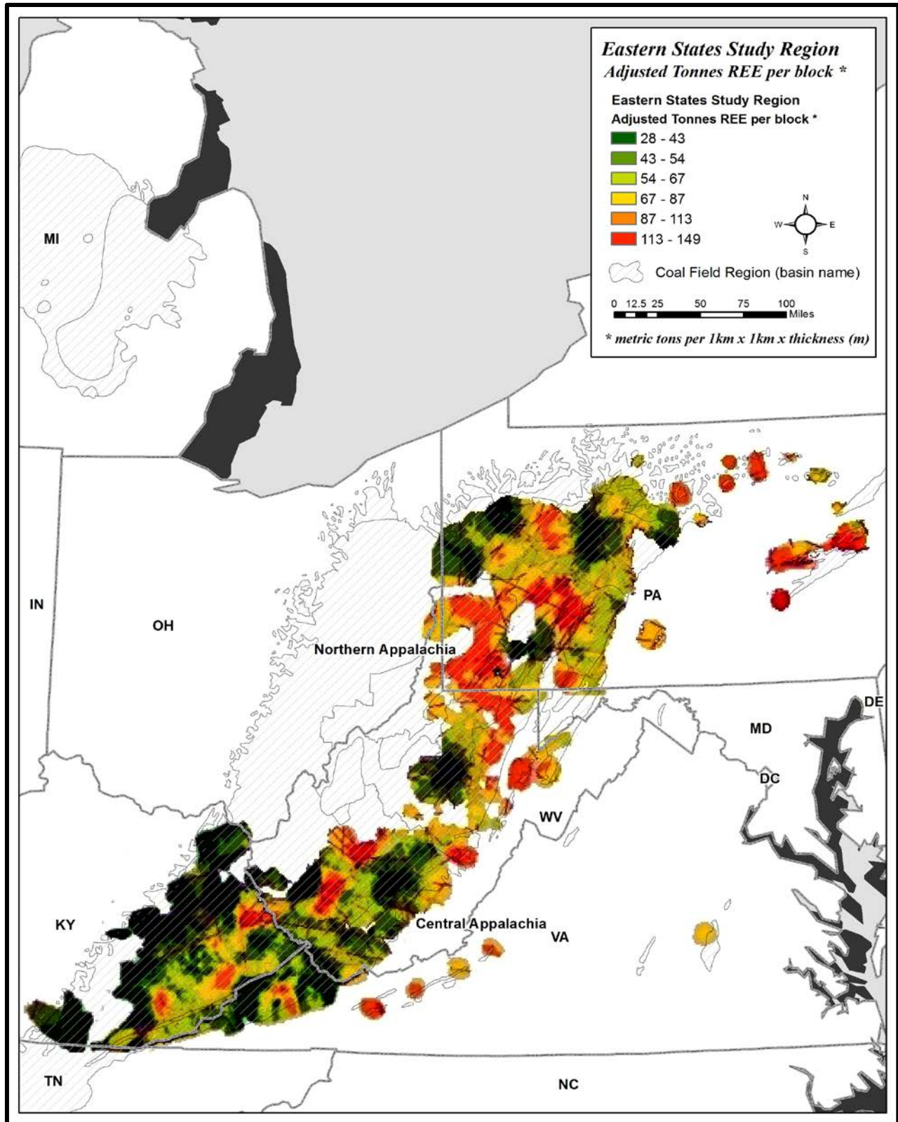
Figure 5b. REEs in U.S. Coal. (b) Map for Appalachian Region.
