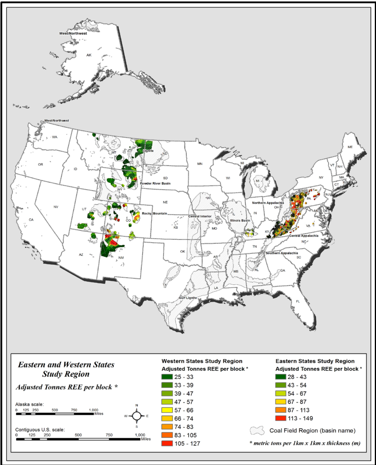
Figure 5a. REEs in U.S. Coal. (a) Map of the continental U.S. (Alaska not analyzed).
