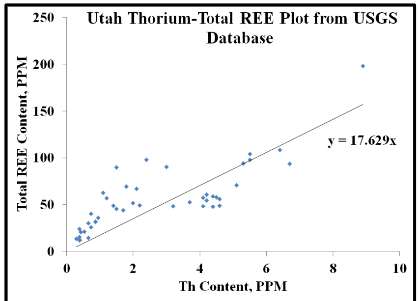
Figure 11a. Thorium-total REEs cross plot
