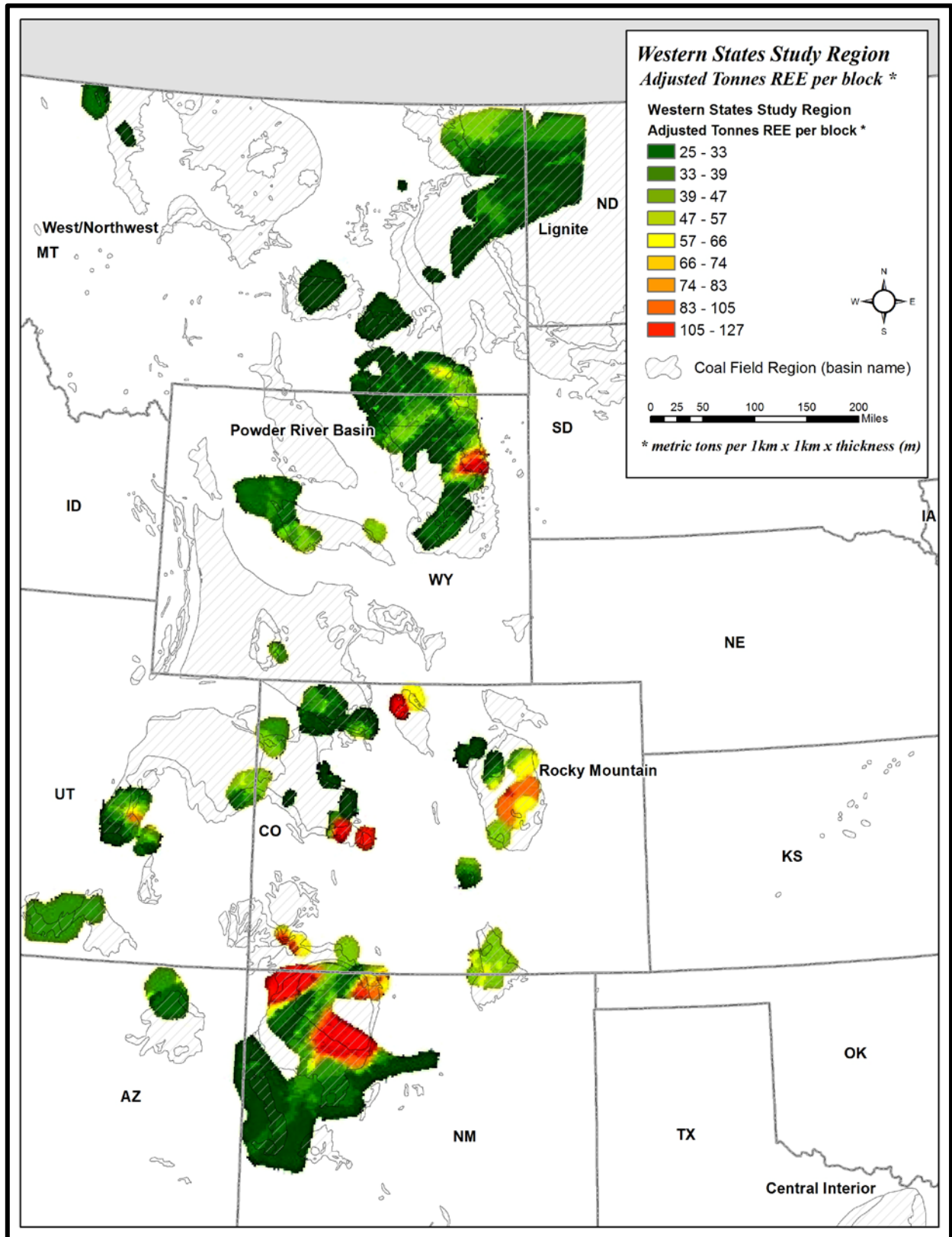
Figure 5c. REEs in U.S. Coal. (c) Map for central and northern Rocky Mountain region.
